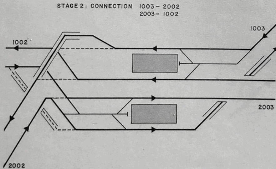
Figure B3-12: Final Design of Flexible Interchange for Station 1001.
